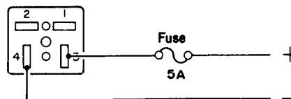
DC Plug connections for external DC supply
