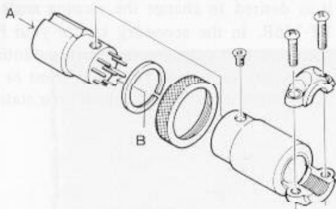
PLUG ASSEMBLY
